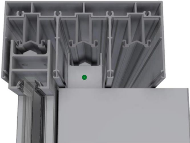
Panel installed in head track. Drill pilot hole prior.
