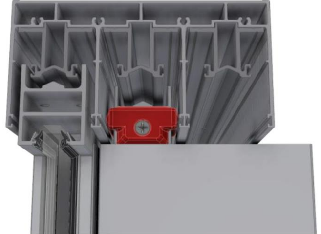
Fit component (shown RED) onto panel, snugly between head track walls.
