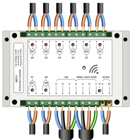
8 Channel Controller
