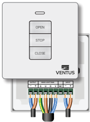
1 Channel Controller
